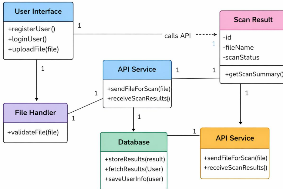
Antivirus File Scanner Application; Class Diagram
